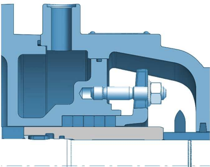
Packet gland cooled with external jacket cooling
