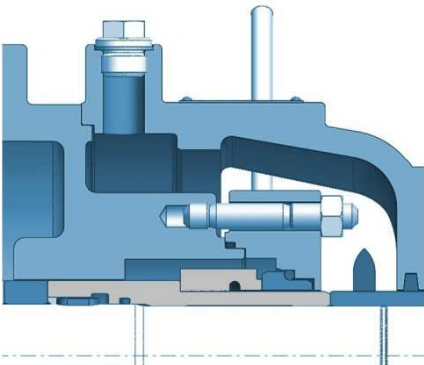
Mechanical seal unbalanced un-cooled with internal feed,
