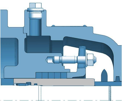
Packet gland un-cooled
