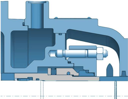
Mechanical seal balanced cooled with external jacket cooling
