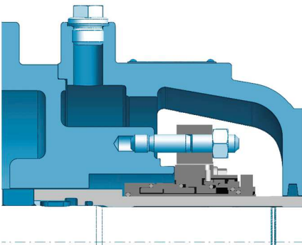
Option: Cartridge seal
