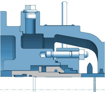
Mechanical seal balanced, un-cooled with internal feed
