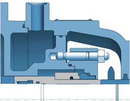
Mechanical seal unbalanced, cooled with external jacket cooling
