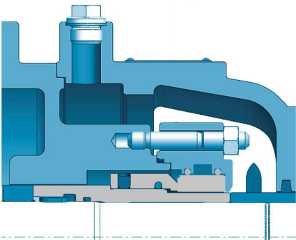
Option: Mechanical seal with counter ring cooling
